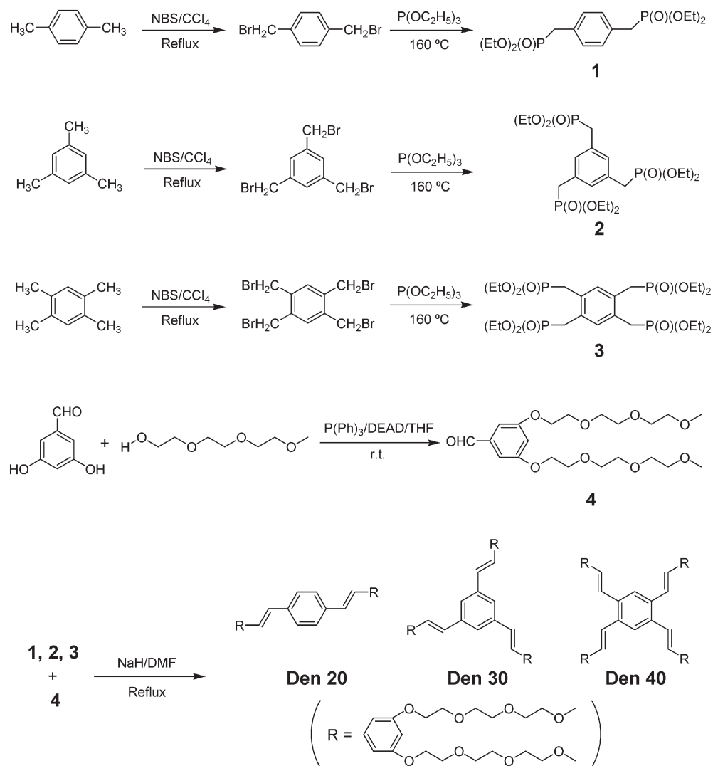
Scheme 1 Procedures for the synthesis of amphiphilic dendrimers with oligo( p -phenylene vinylene) core units and oligo(ethylene oxide) terminal chains.
